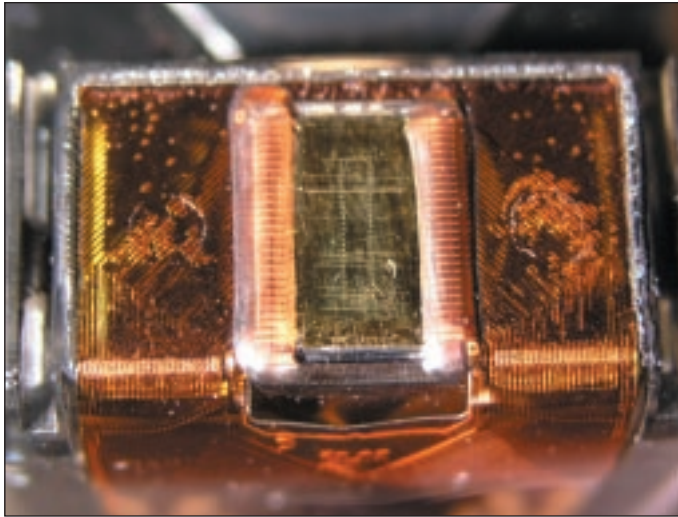
Figure 2c. Optical microscopy of used HP 629A cartridge with scratches on the nozzle plate.
