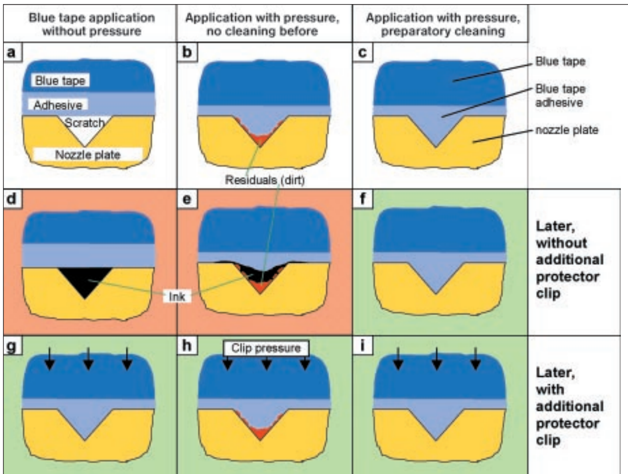
Figure 6. Schematic representation of the different possibilities for ink cartridge sealing. 6a, 6b and 6c: Three possibilities of blue tape application, just at the moment of application. 6d, 6e and 6f: Cartridge storage with blue tape, but without additional protector clip. 6g, 6h and 6i: Cartridge storage with blue tape and with additional protector clip.
