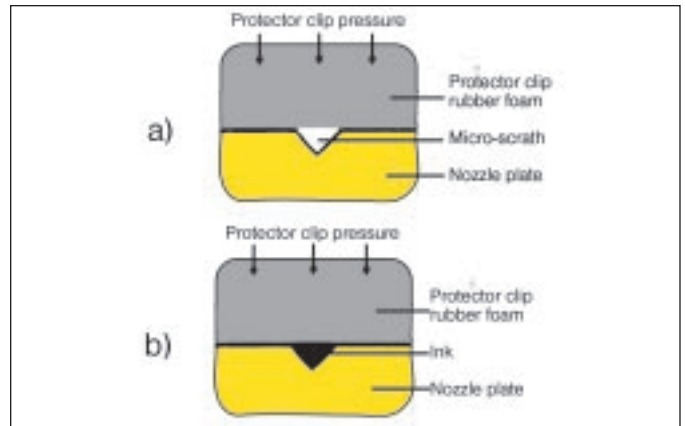
Figure 5a. Schematic representation of a transverse cut of a nozzle plate surface containing a micro-scratch. There is a protector clip applied from above causing a permanent pressure on the rubber foam (gray) and consequently on the nozzle plate. Figure 5b. Formation of a channel between rubber foam and nozzle plate containing air. Cartridge storage causes filling of the micro-scratch with ink by capillarity.
