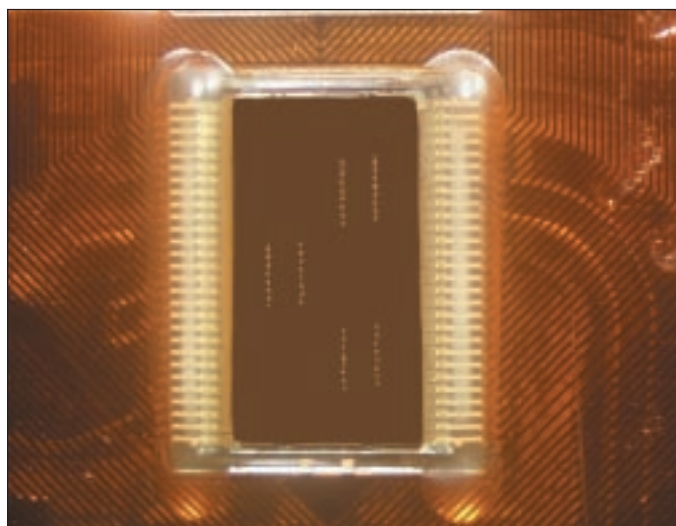
Figure 2a. Stereo microscopy showing print heads and nozzle plates of a new HP 625A cartridge.
