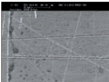
Figure 3. Scratch network on the nozzle plate surface of a used cartridge.
